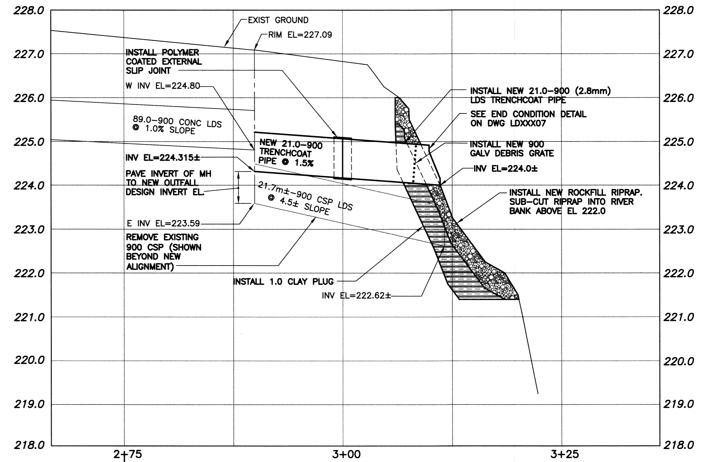
CRANE AVENUE NEW OUTFALL (RR-27) PROFILE
