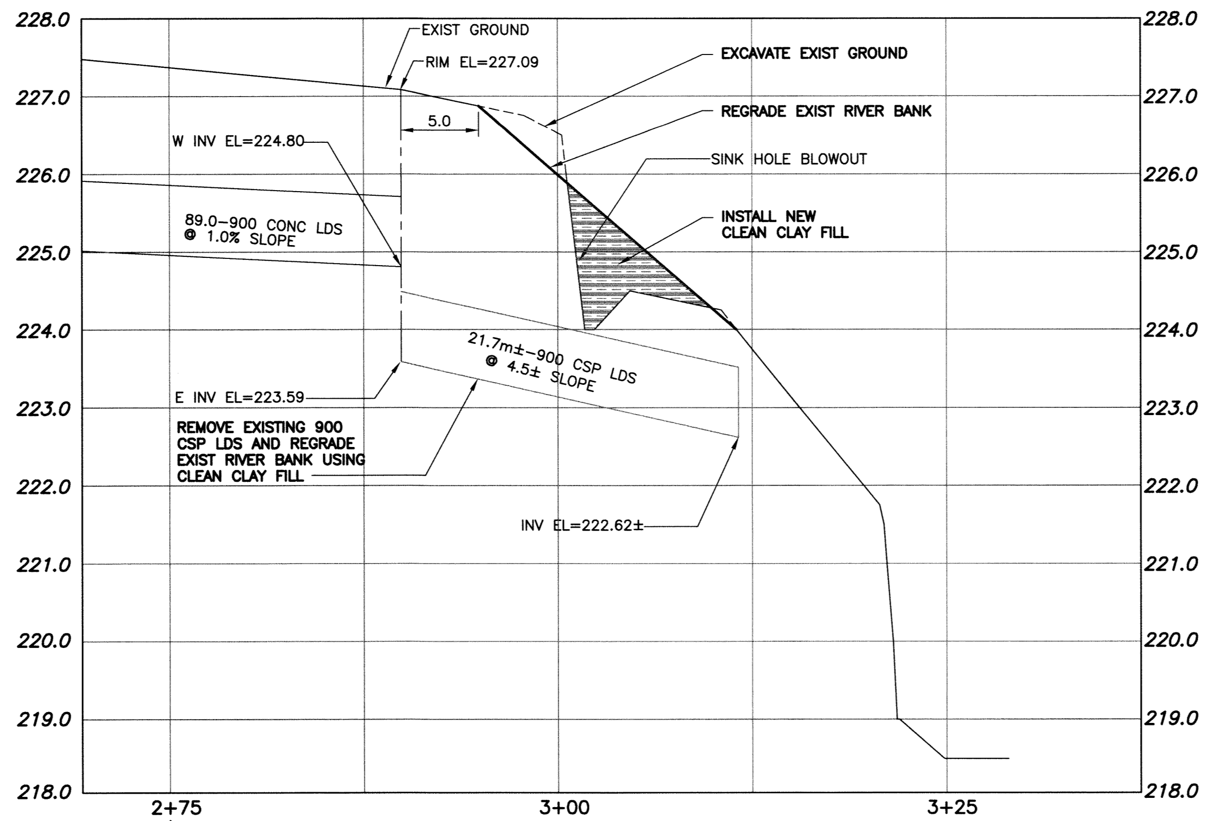
CRANE AVENUE EXISTING OUTFALL (RR-27) PROFILE
